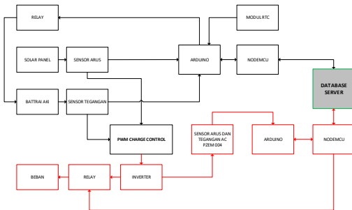
Gambar 6. Perancangan Hardware
