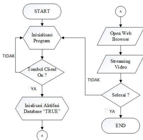
Gambar 3. Flowchart
