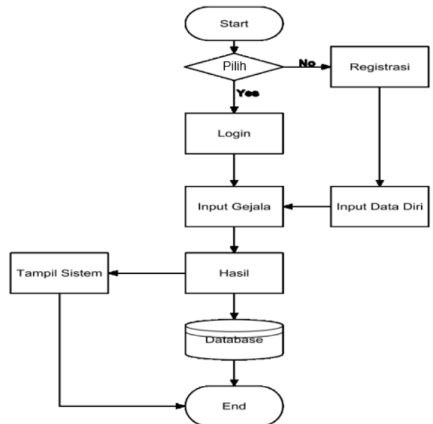
Gambar 1. Flowchart User
