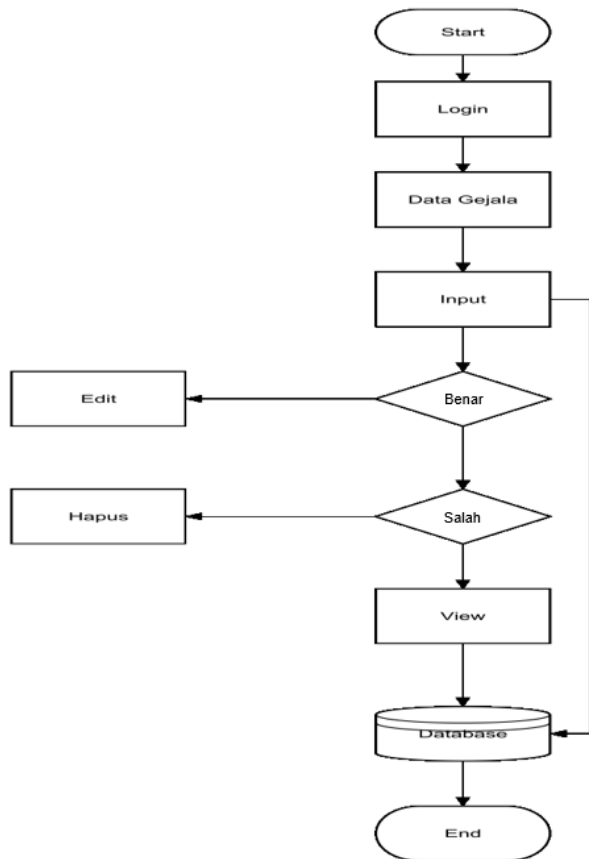
Gambar 2. Flowchart Admin
